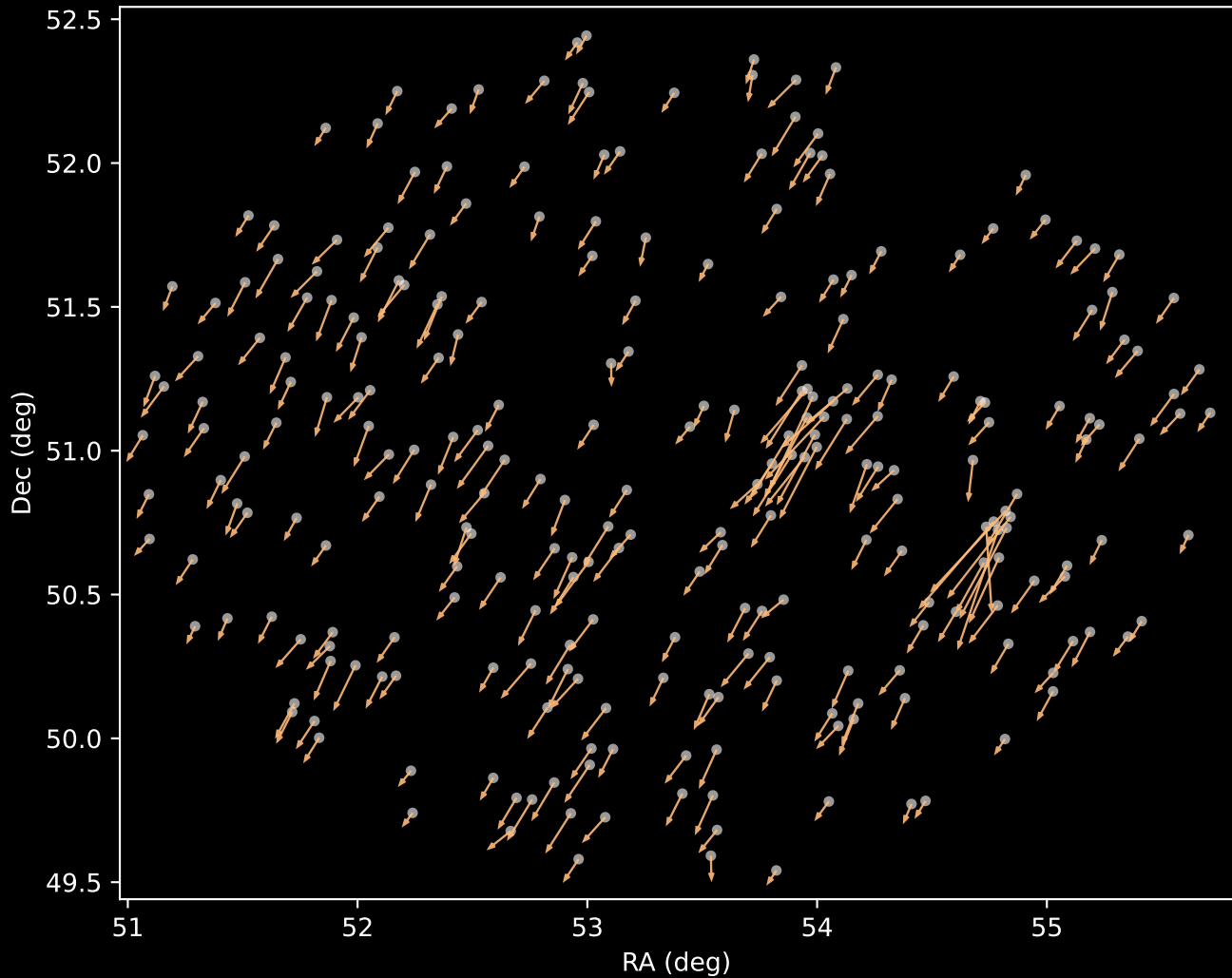
APOGEE DR17 Cluster 3 Proper Motion Vectors (n=260)
