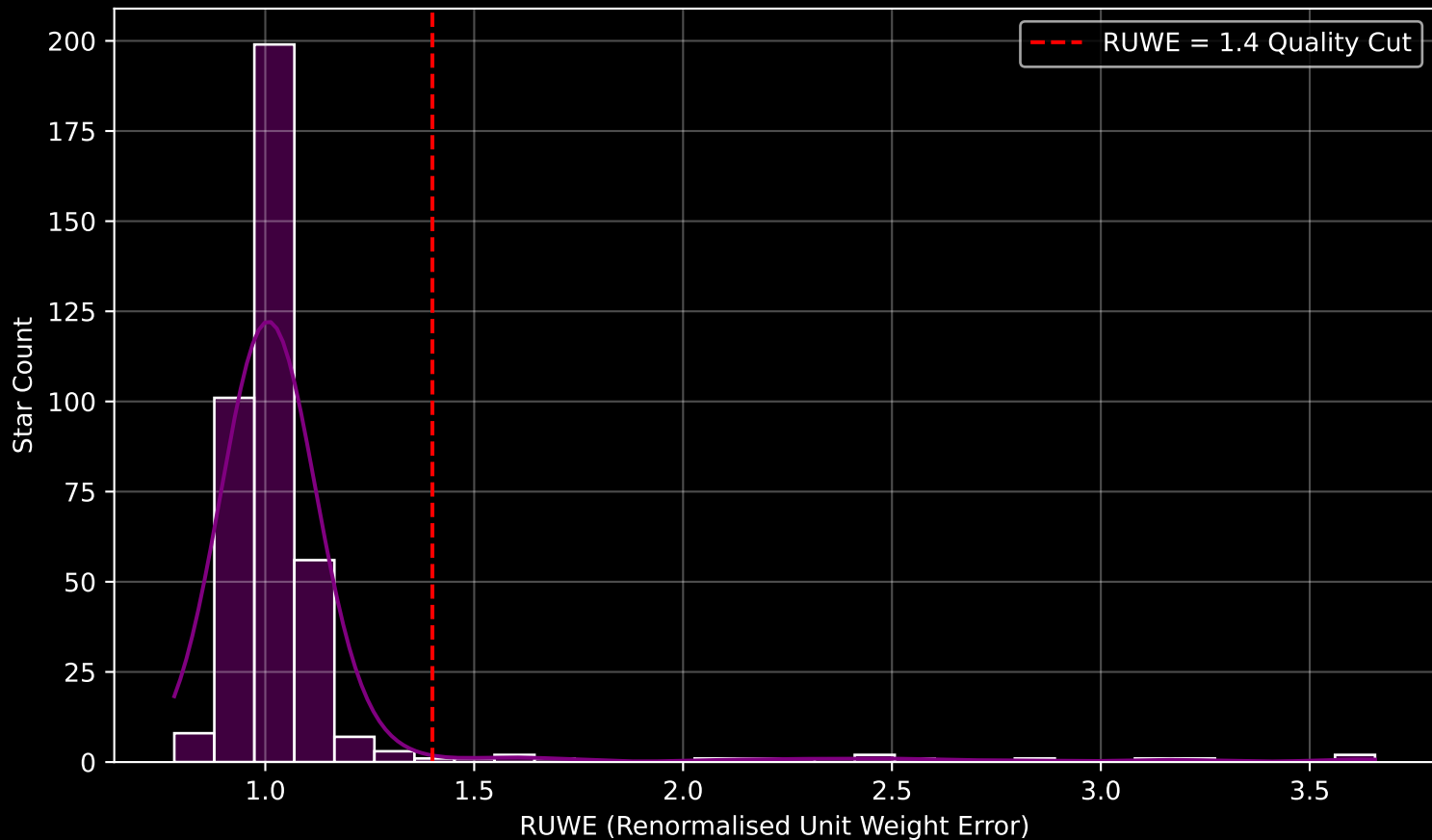
GAPOGEE DR17 Field [090+04] RUWE Distribution (n= 390)
