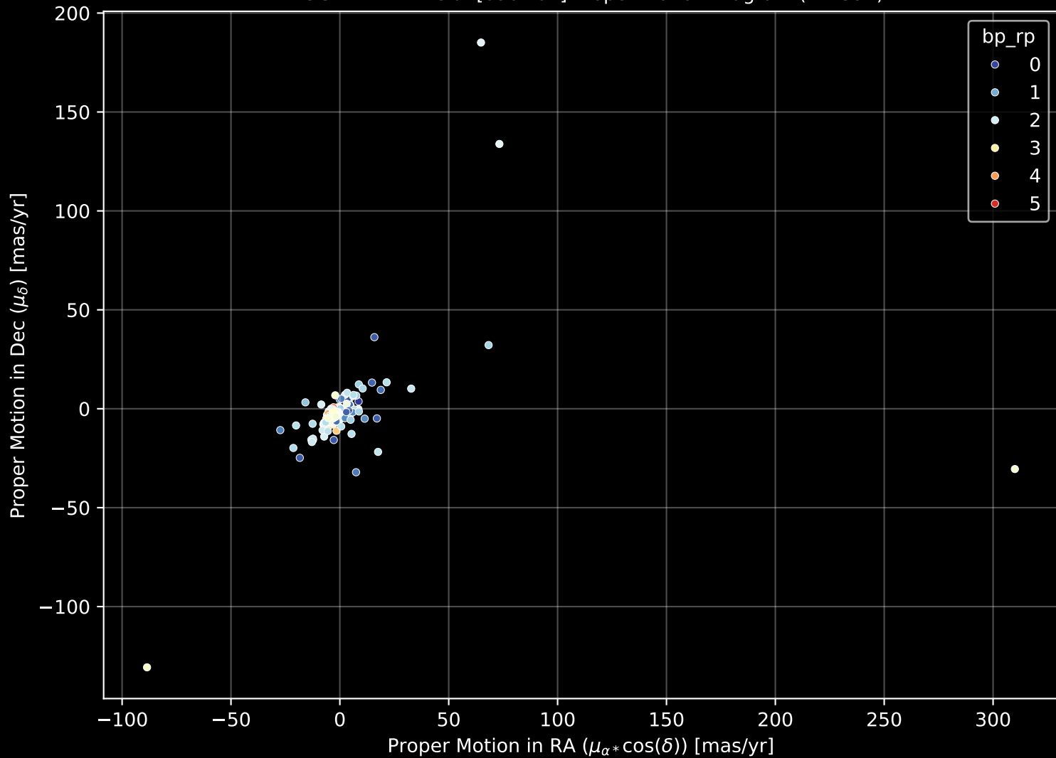
APOGEE DR17 Field: [090+04] Proper Motion Diagram (n= 397)
