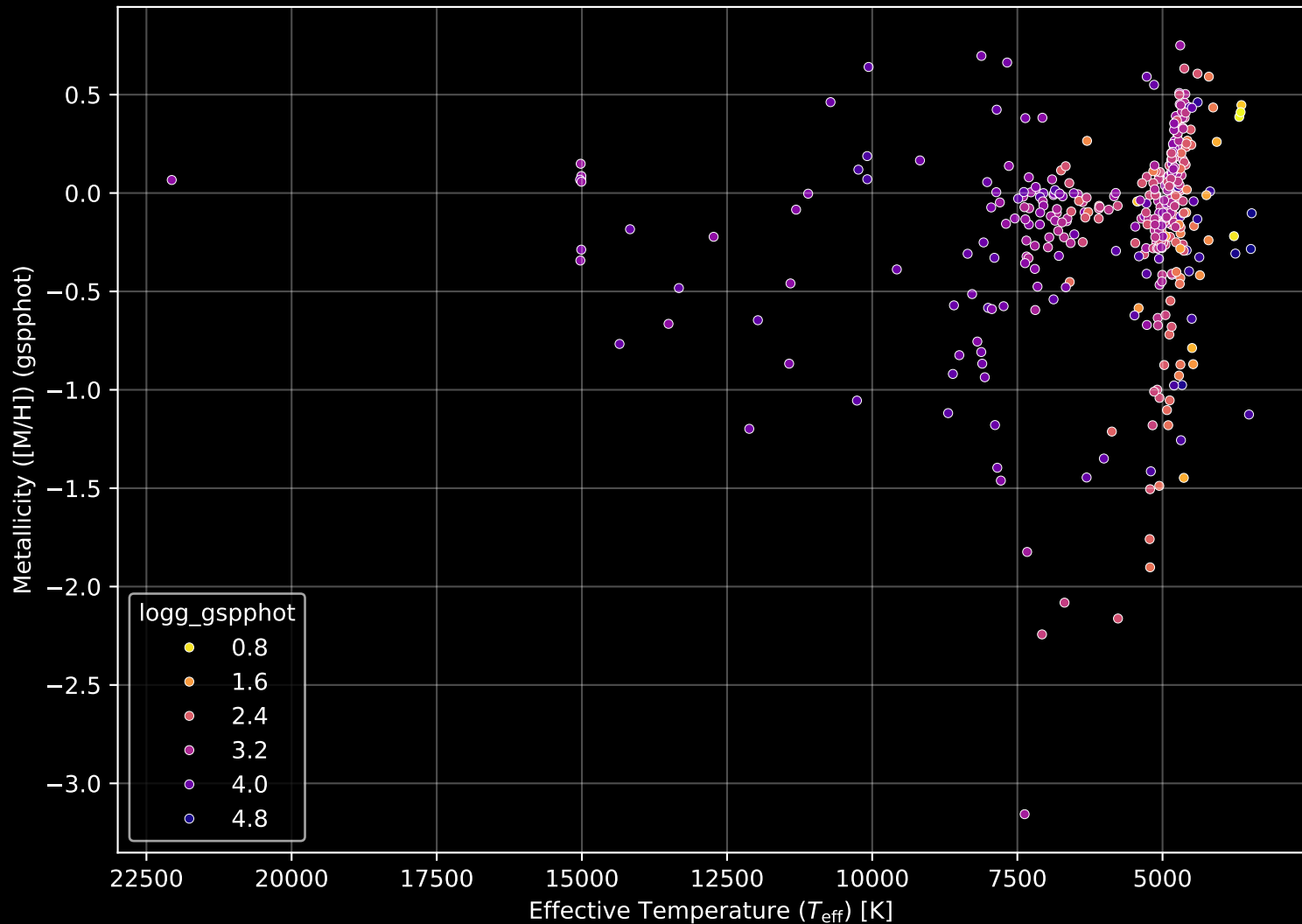
APOGEE DR17 Field: [090+04] Stellar Population Parameters (n= 397)
