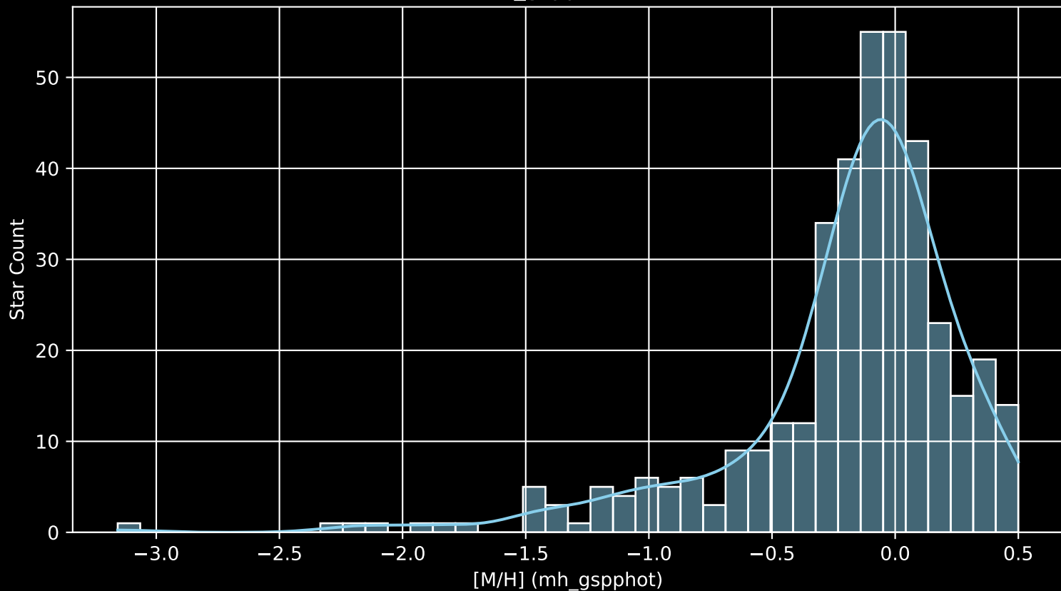
APOGEE DR17 Field: [090+04 [M/H] (mh_gspphot) (n= 386)
