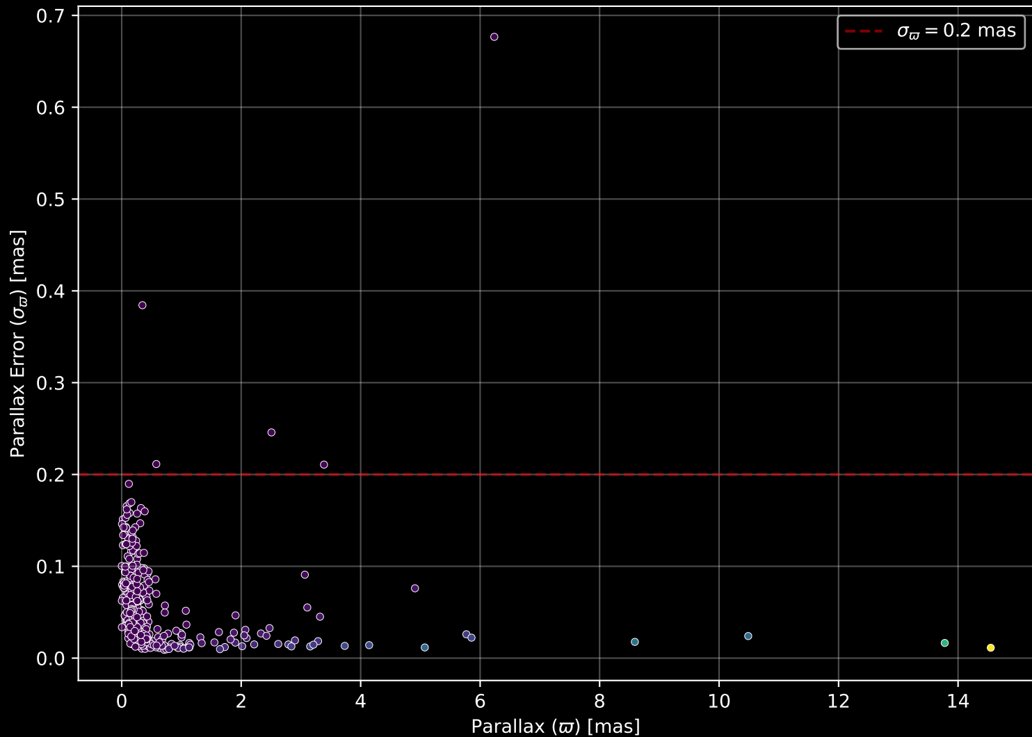
APOGEE DR17 Field: [090+04] Parallax Quality (n= 397)
